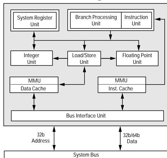
PowerPC 603e Microprocessor Block Diagram
